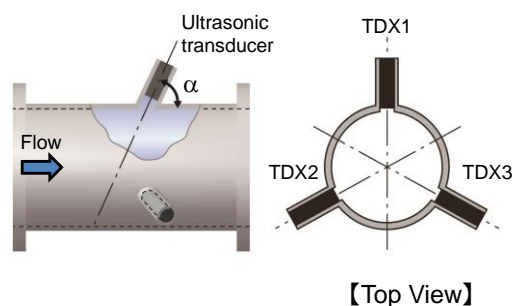
Figure 1: Test section
