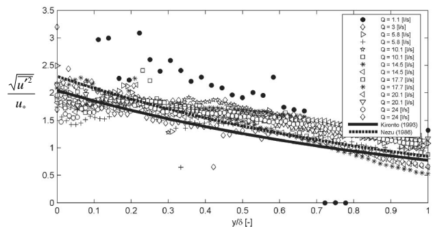
Figure 3: Dimensionless distribution of horizontal turbulence intensity \sqrt{u'^2}/u_s(y) for different flow conditions.
