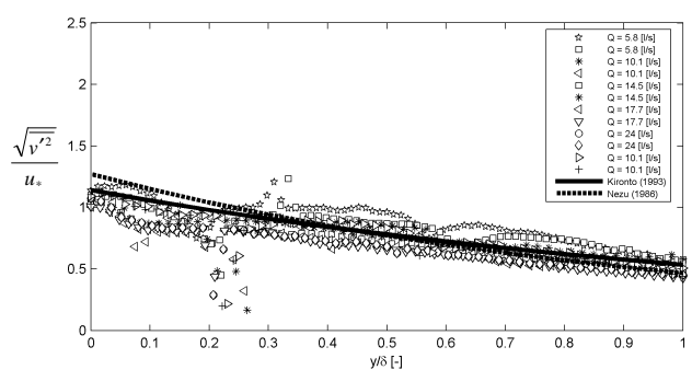
Figure 4: Dimensionless distribution of horizontal turbulence intensity \sqrt{v'^2}/u_s(y) for different flow conditions.
