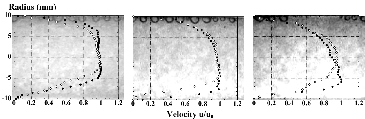
Fig. 3 : Variation of the particle velocity profiles depending on the mass flow. From the left to the right: 0,21 kg/s, 0,09 kg/s, 0,06 kg/s. Black pointers show vertical profiles and white ones belong to horizontal profiles. In the background ice slurry particles flowing through the tube can be recognized.
