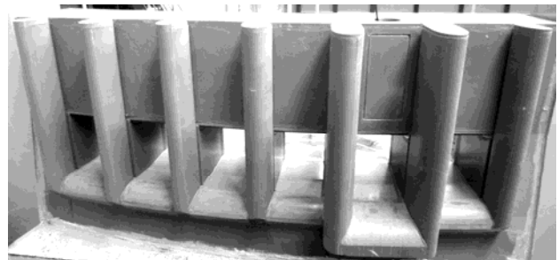
Figure 1: Physical model of orifice spillway seen from reservoir, considered gate is second from right
